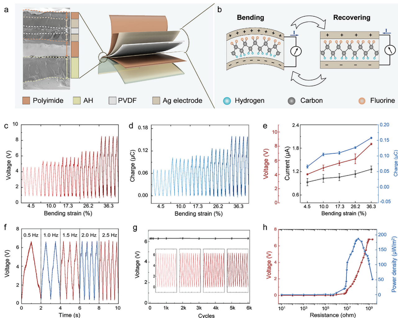
Figure 4. In vitro electrical performance of TPSS. a) The SEM and explosive view of TPSS displayed the multi-layered structure with close contact between layers. b) The working principle of TPSS. c) The V_{OC} and d) C_{SC} of TPSS under different bending strains. e) The V_{OC} , I_{SC} , and C_{SC} of TPSS vary with different bending strains. f) The V_{OC} of TPSS under different frequencies with the bending strain fixed at 26.2%. g) The V_{OC} and power density of TPSS in an impedance-matching test. h) The performance stability of TPSS with 6000 times bending-recovering test under the 26.2% bending strain.
