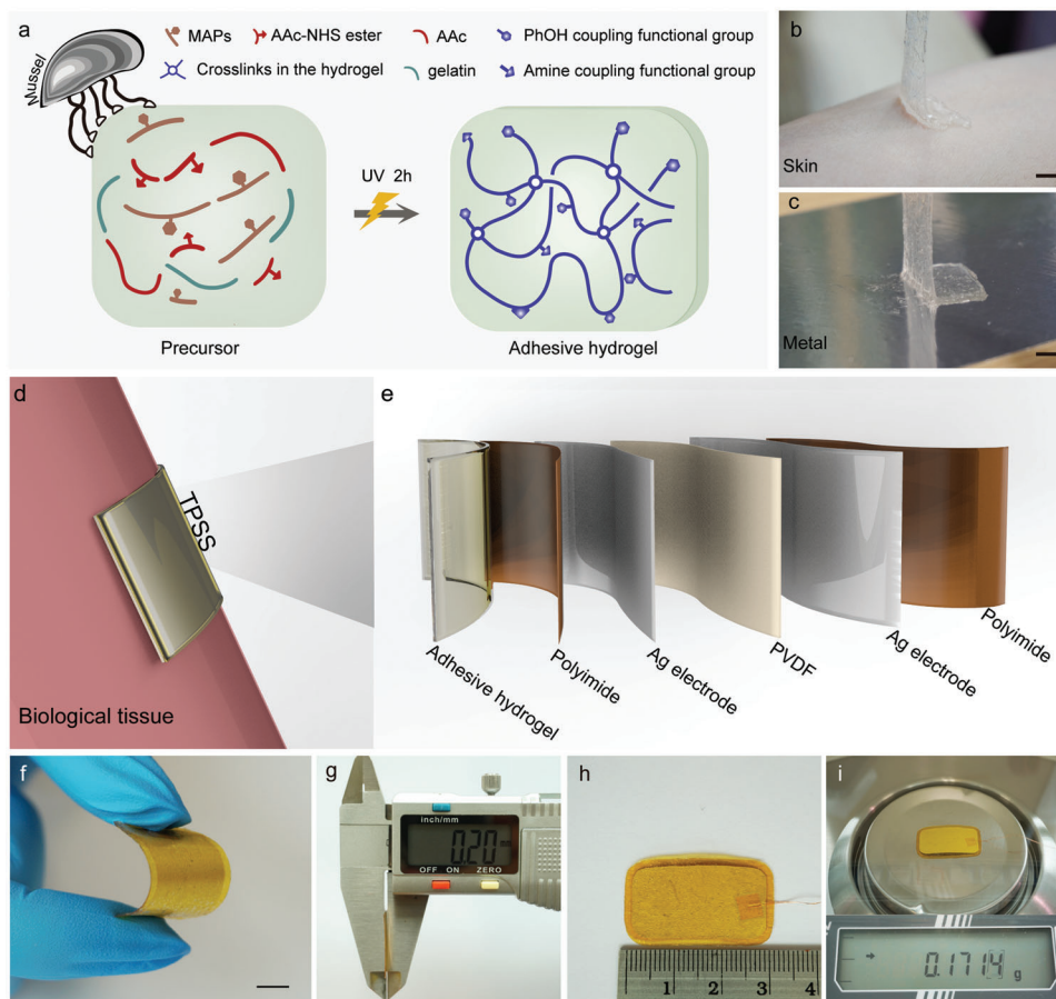
Figure 1. The overview of TPSS. a) The design process, components, and structure of AH. b) The AH adhered to the skin. c) The AH adhered to metal (Al film). Scale bars in (b) and (c) both are 1 cm. d) The diagram of TPSS in vivo, with the help of the AH, the TPSS anchor at the implant site. e) An exploded view of TPSS. f–i) The optical images of the TPSS in well flexible with a dimension of 30 \times 15 \times 0.2 \text{ mm}^3 , and a weight of 0.171 g. Scale bar: 1 cm.
