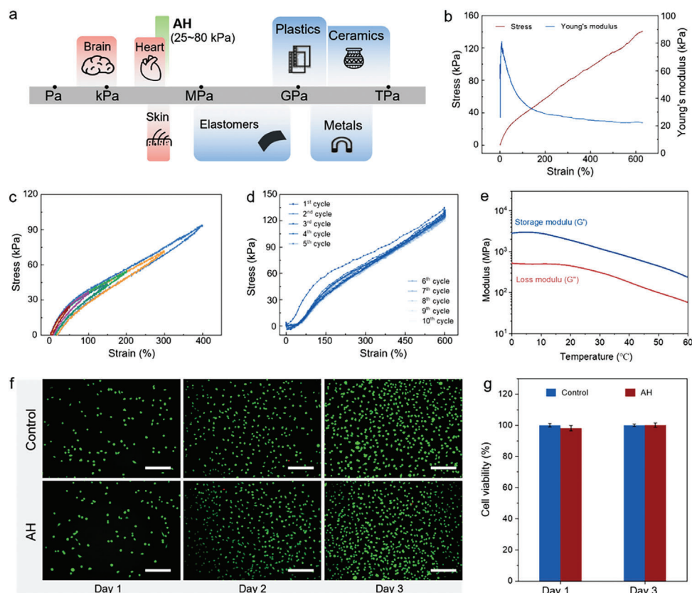
Figure 3. The mechanical performance and biocompatibility of AH. a) Young's modulus of AH is in the range of \approx 25 –80 kPa, which is located between engineering materials and biological tissues. b) The tensile strain-stress curve and Young's modulus curve of AH. c) The loading-unloading tensile strain-stress curves of AH with maximum tensile deformation fixed at 50%, 100%, 150%, 200%, 300%, and 400%. d) The 10 times loading-unloading tensile strain-stress curves of AH with maximum tensile deformation fixed at 400%. Loading speed in (c) and (d) was 30 \text{ mm min}^{-1} . e) The storage modulus ( G' ) and loss modulus ( G'' ) of AH under temperatures ranging from 0 to 60 °C. f) The fluorescence images and g) cell viability of stained mouse embryo fibroblasts after being cultured with AH for 1, 2, and 3 days. The scale bar in (f) is 200 \mu\text{m} .
