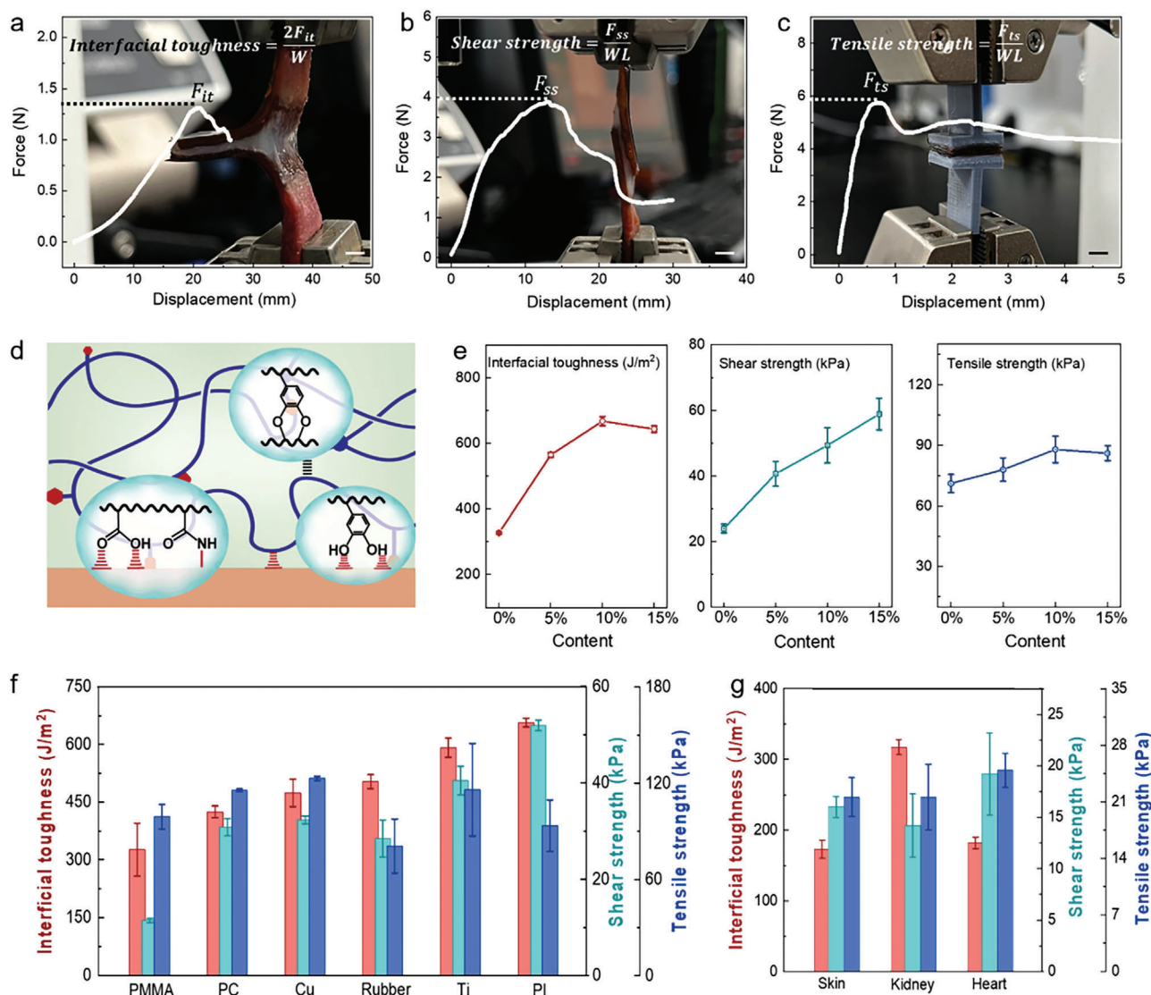
Figure 2. Mechanical adhesion performance of AH. The adhesion abilities of AH were evaluated by three methods: a) interfacial toughness tested by a standard 180° peel test, b) shear strength tested by a standard lap-shear test, and c) tensile strength tested by a standard tensile test. The biological targets used in (a–c) were small pieces of the kidney. Scale bar in (a–c) is 1 cm. d) The adhesion principle of AH. e) The interfacial toughness, shear strength, and tensile strength of AH (with PI as test targets) vary with the content of MAPs. f) Interfacial toughness, shear strength, and tensile strength between AH and various engineering materials. g) Interfacial toughness, shear strength, and tensile strength between AH and biological tissues. The loading speed of all tests was 30 mm min −1 .
