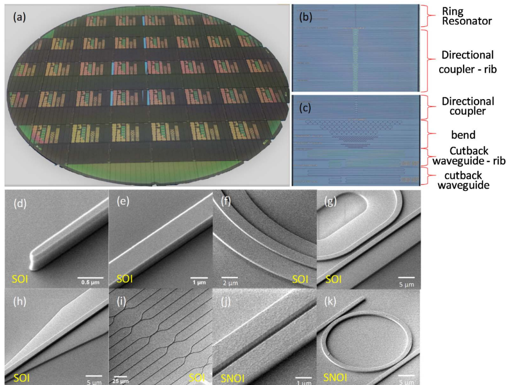
Fig. 2. (a) Fabricated 8-in. silicon wafer with MIR devices after wafer dicing for characterization. (b) SOI strip ring resonators and rib DCs. (c) SOI strip DCs, bends, waveguides, and rib waveguides. (d)–(k) SEM images of the fabricated devices. (d) SOI waveguide taper tip. (e) SOI strip waveguide. (f) SOI rib waveguide. (g) SOI rib DC. (h) SOI strip to rib converter. (i) SOI strip DC array. (j) SNOI DC. (k) SNOI add-drop ring resonator.
