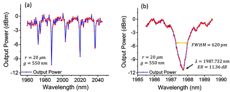
Fig. 7. Characterization of the SNOI strip ring resonator with radius of 20 \mu\text{m} and coupling gap of 550 nm. Transmission spectrum of the ring resonator (a) from 1960 to 2045 nm with scanning step of 0.54 nm (b) around the resonance of 1988 nm with scanning step of 0.011 nm.
